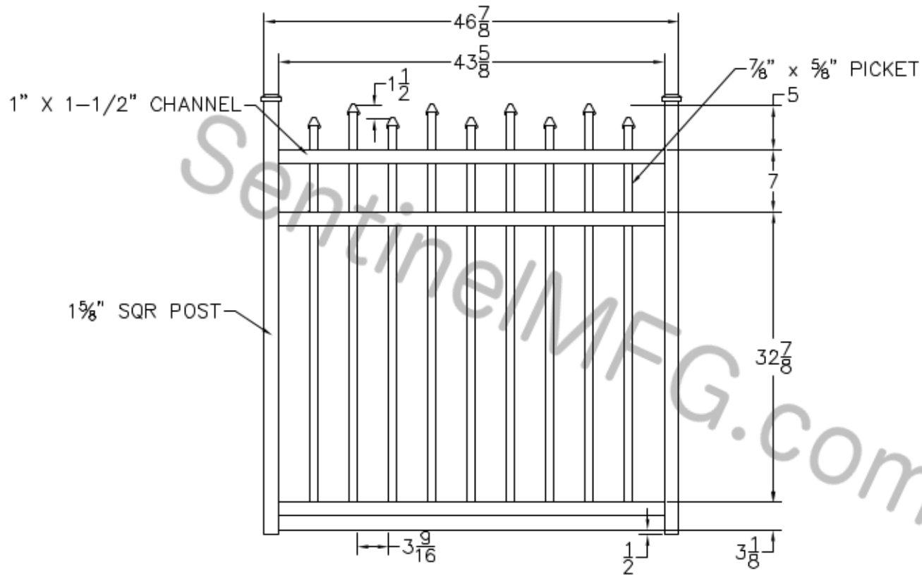
OUTSIDE VIEW
